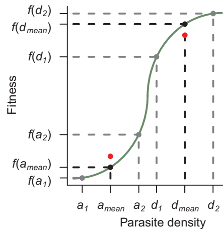
Figure 1: When fitness is a convex function of density (e.g., the a values in the accelerating part of the curve), oscillations in density can increase mean fitness as a consequence of Jensen's inequality (reviewed in Ruel and Ayres 1999). A strain that alternates between densities a_1 and a_2 has higher mean fitness (red point) than a strain that maintains a constant density a_{\text{mean}} (black point). If fitness is a concave or decelerating function of density ( d values), oscillations in numbers decrease mean fitness compared to a strain that maintains a constant density (red vs. black point). Cumulative fitness is altered in an identical manner.
